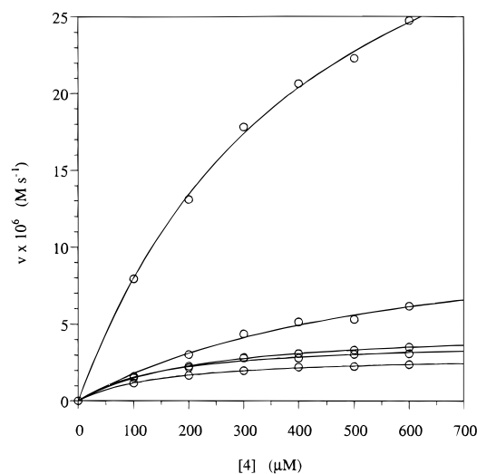
Figure 2. V vs [S] plots for the antibody-catalyzed isomerization of 4 to 6 . Data were fit to the Michaelis–Menten equation v = V_{\max} [4]/(K_M + [4]) . The rates v were normalized to the protein concentration after being corrected for the background reaction. The antibodies are, from the top to the bottom, 64D8E10 (0.26 \mu\text{M} ), 56D10D6 (1.3 \mu\text{M} ), 51F3D2 (3.3 \mu\text{M} ), 83F12D6 (4.2 \mu\text{M} ), and 83F11C4 (4.9 \mu\text{M} ).
